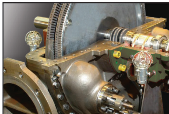
Typically, two Sentinel FBSs are installed in each gland box to provide superior sealing while protecting downstream carbon rings from contamination and high pressure.
